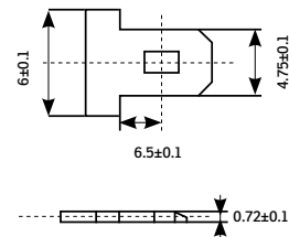
Terminals T1 (F1)
